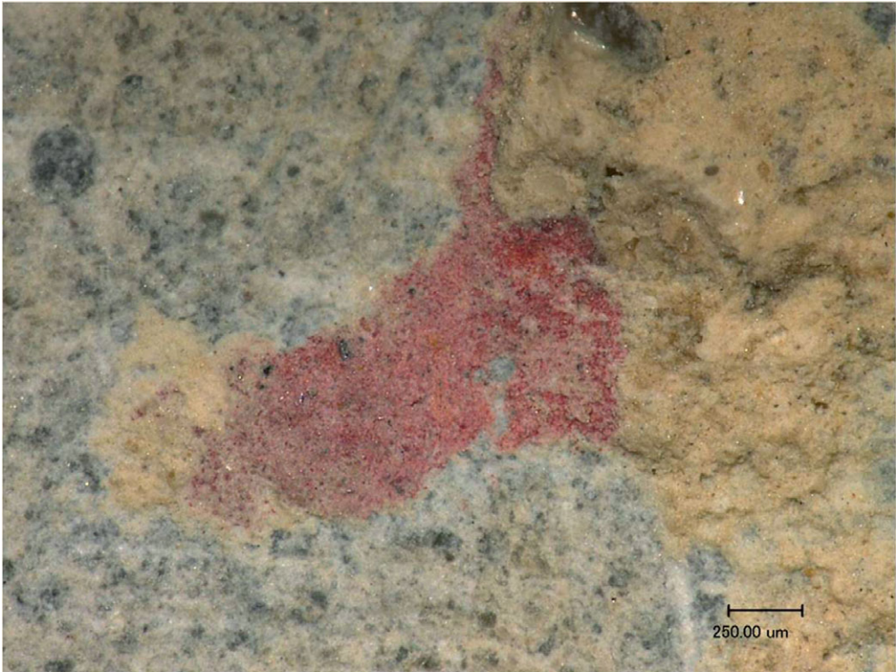
3.12. Tripylon, north, eastern door jamb, detail. Photomicrograph: M. Pamplona
